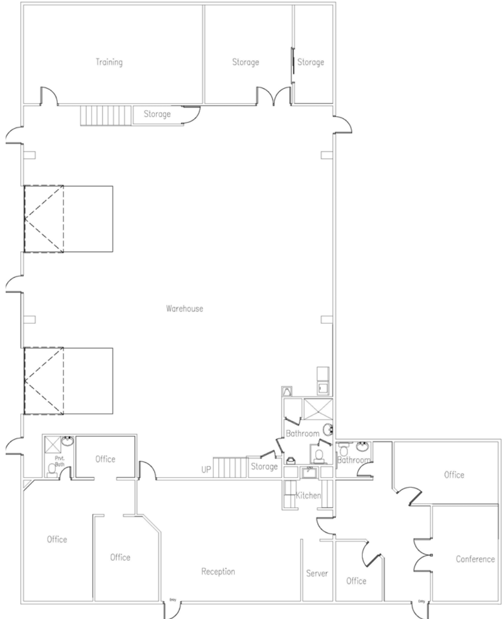
FIRST FLOOR SCALE: \frac{1}{8}'' = 1'-0''
