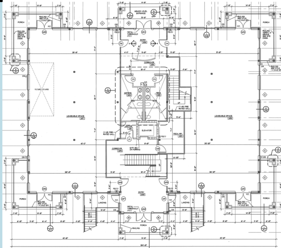
FLOOR PLAN - SECOND FLOOR SCALE: 3/8" = 1'-0"
