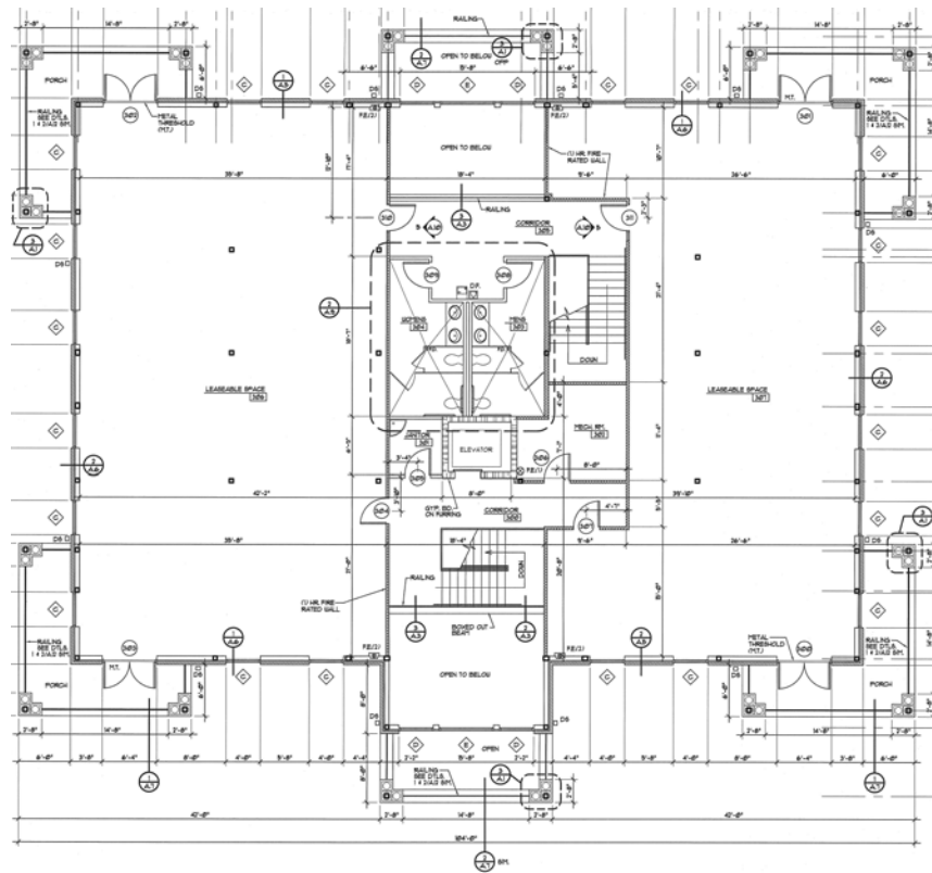
FLOOR PLAN - THIRD FLOOR SCALE: 3/8" = 1'-0"
